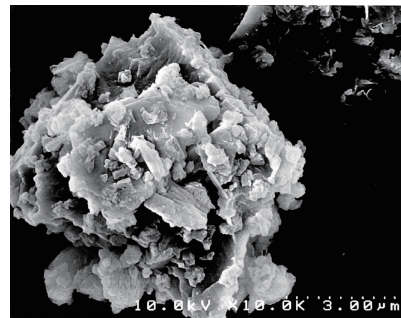
Fig. 2 An electron micrograph of a shirasu grain. *The total surface area of shirasu per 1 gram is approx. 9m 2
