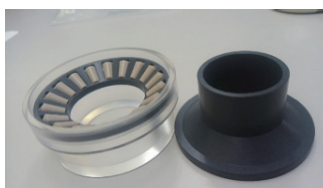
PTFE thrust bearing
